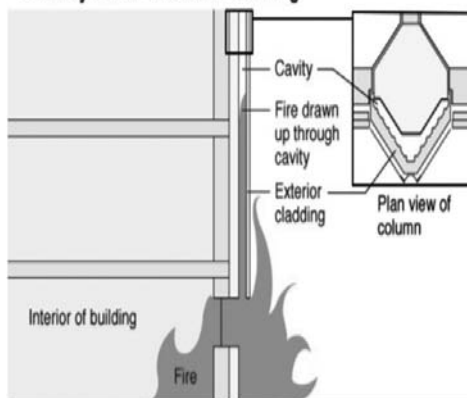
"Chimney effect" of exterior cladding
