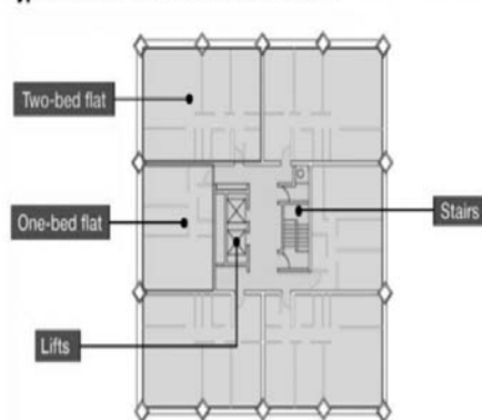
Typical residential floor in Grenfell Tower
